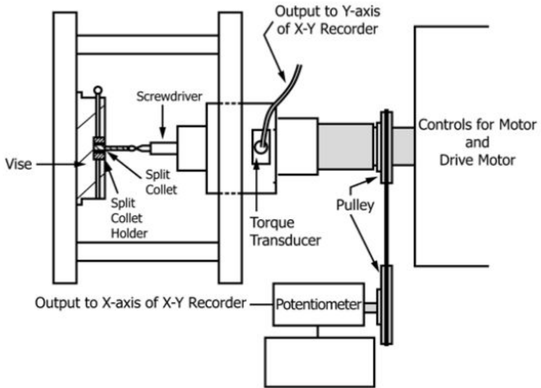
Fig: Representative test setup
